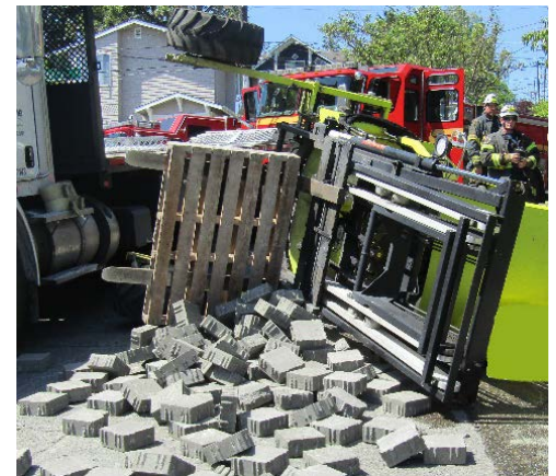
Scene where delivery driver was pinned under the forklift's overhead guard when it overturned on a 20-degree slope.
